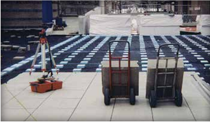
Figure 6. Foam pedestal system
